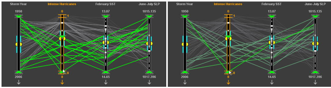
Figure 3: An example of the discrete (left) and continuous (right) modes of the aerial perspective shading capability. Lines are shaded based on their position relative to the axis focus, context, and query areas and, in continuous mode, a nonlinear color gradient effect encodes the distance to the mouse cursor. In these examples, the mouse is positioned over the bottom of the second axis which highlights the seasons with high intense hurricane activity and, in continuous mode, the most active seasons are given more emphasis.
